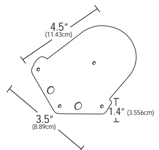
GPS Receiver Bracket Part # 105005
