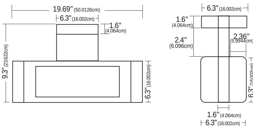
Ceiling Mount - Front View
